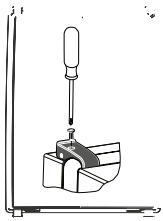
Installing casing
